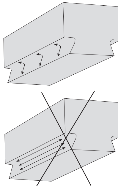
Grinding of dove-tail radii.
